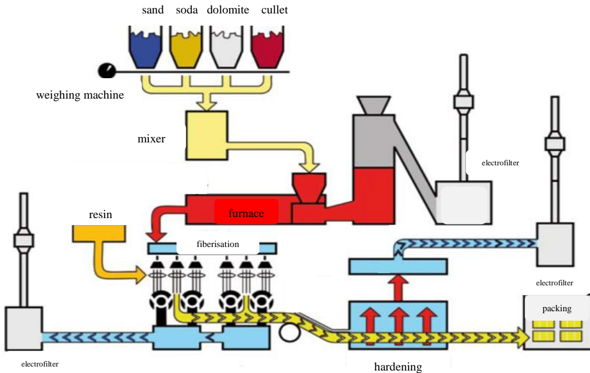
Figure 2. Production scheme for URSA GLASSWOOL
